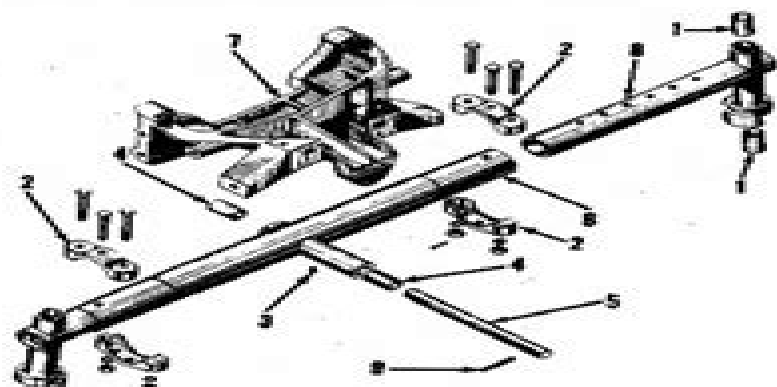
Fig. 1—Exploded view of Series B-275 adjustable front axle and component parts. Bushings (1 and 4) are pre-sized. Shims (10—Fig. 2) are also used with this axle.
