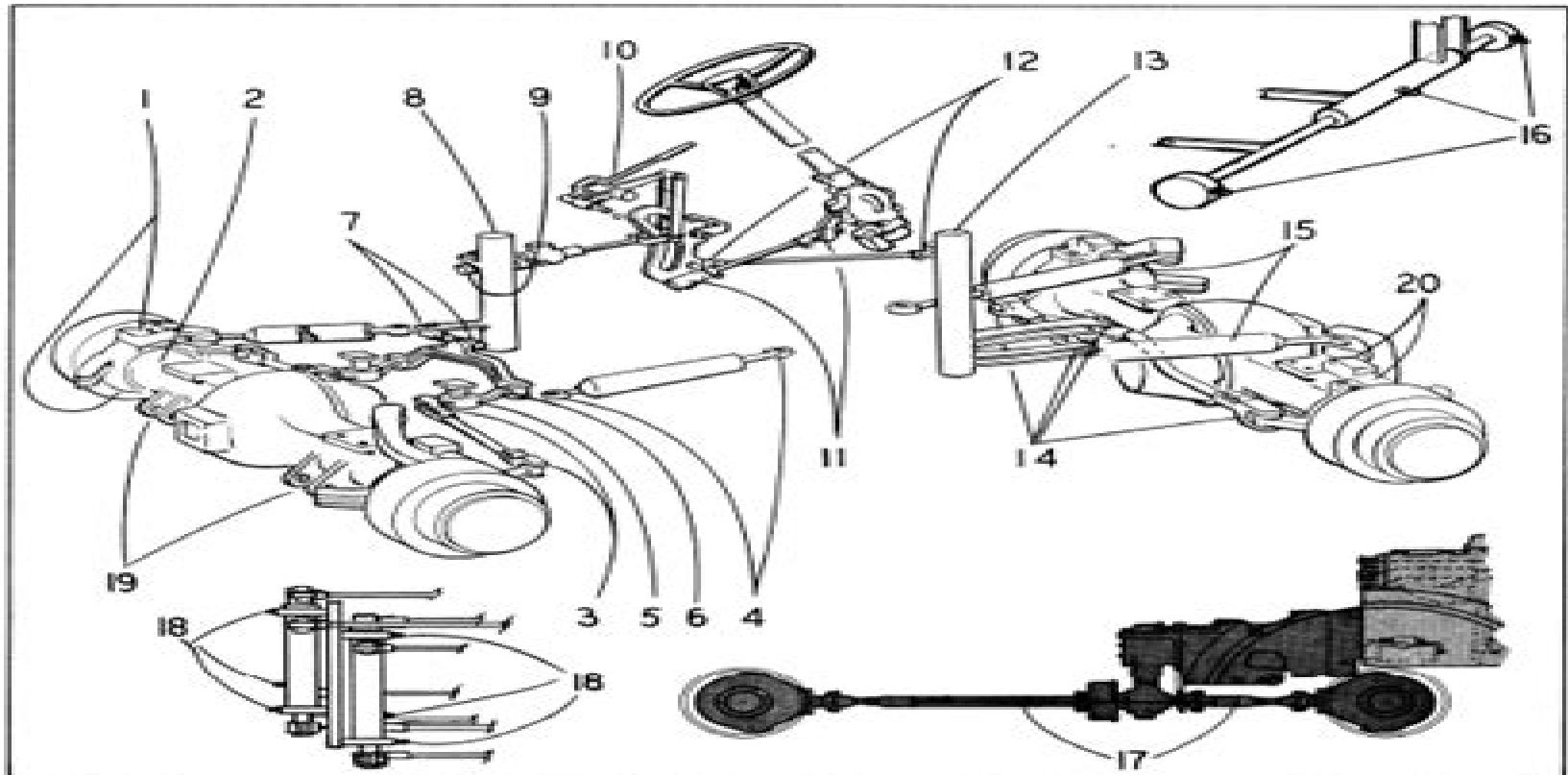
Figure 37. Chassis lubrication diagram
