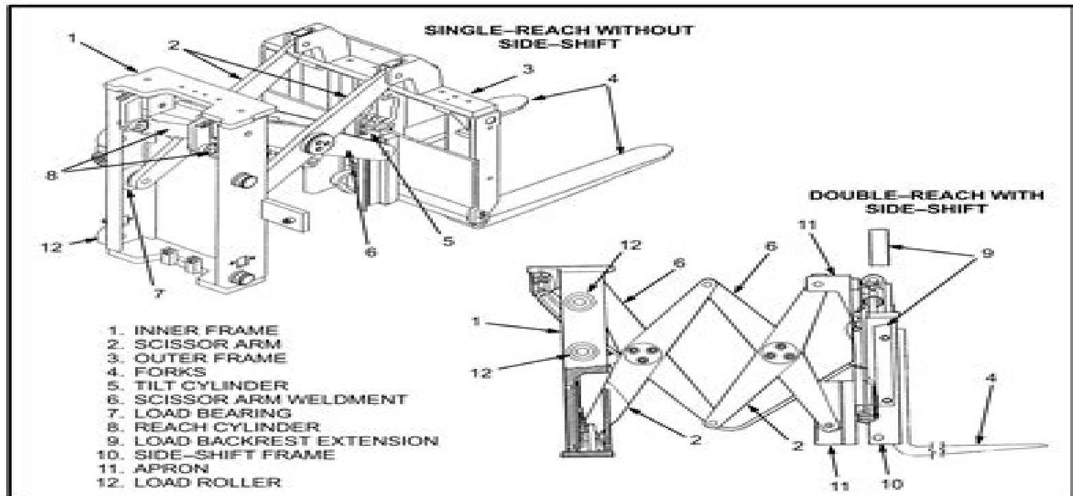
FIGURE 1. REACH CARRIAGES
