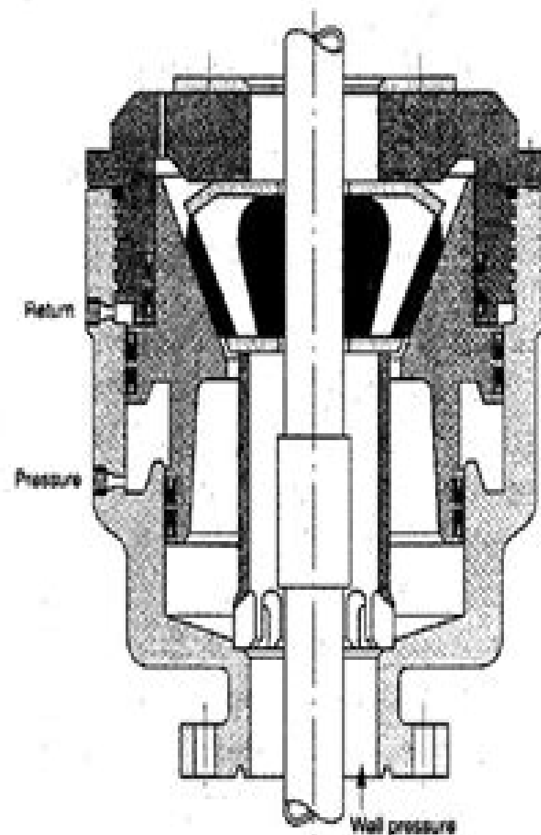
Closed preventer
