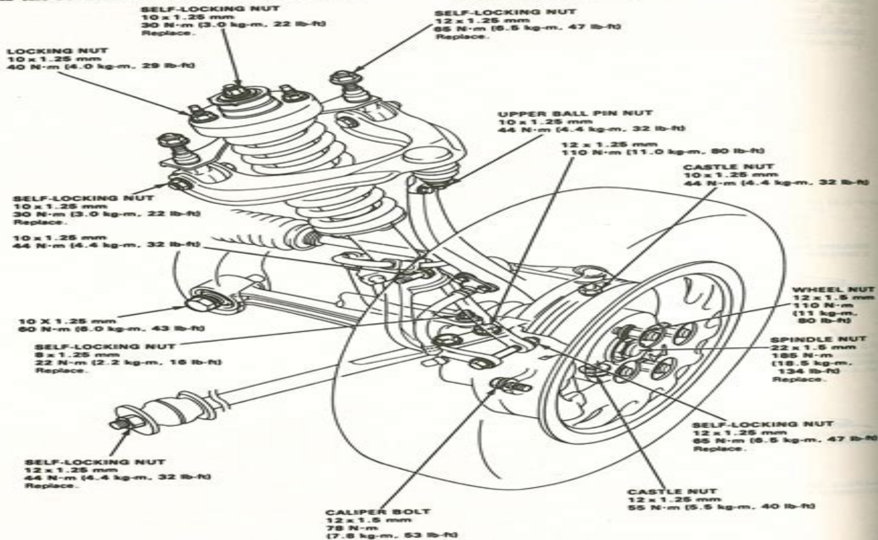
Front suspension fastener locations—1988-91 models
