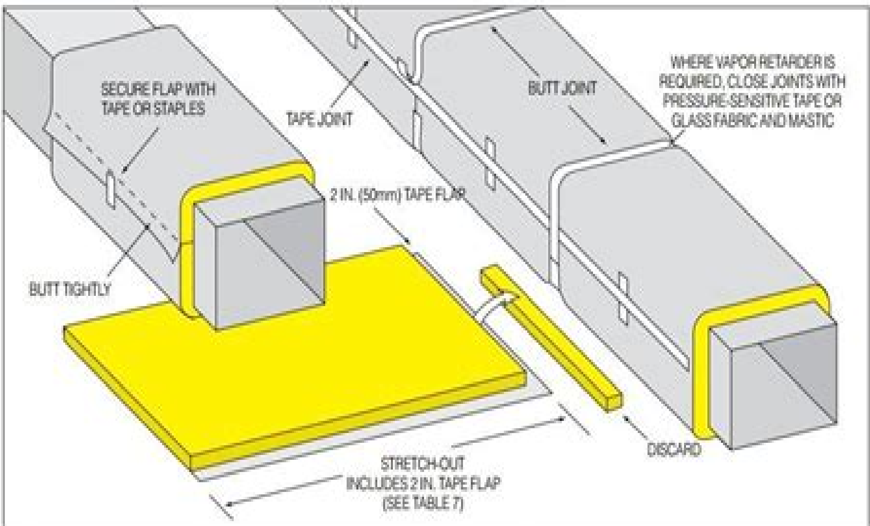
Fig. 23. Installing fibrous glass duct wrap insulation to assure full installed R-value
