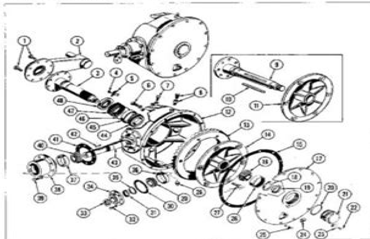
Fig. 1 — Bevel Gear Main Drive Assembly
