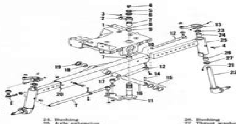
Fig. 1—Exploded view of typical adjustable front axle assembly used on all models. A two-piece steering arm and shaft (13) is used on some models.
