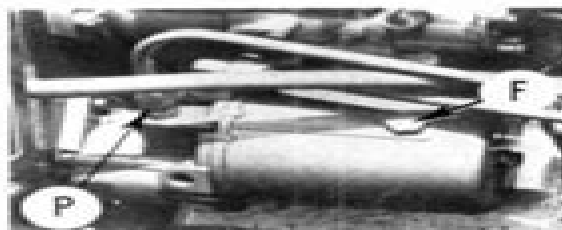
Fig. 2—The power steering reservoir is filled through hole for plug (F). Pump pressure line is shown at (P).
