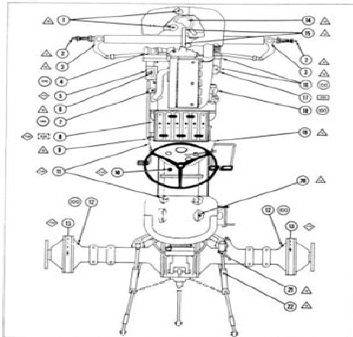
Fig. 1 - Lubrication Chart (Blasal Engine)
