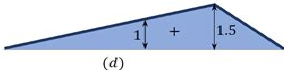
Influence line for reaction B_y
