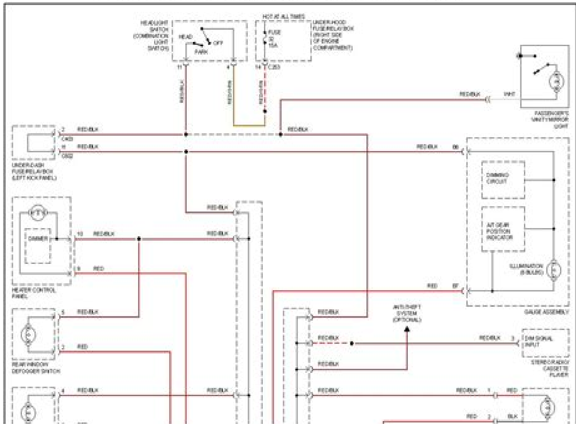
1994 Honda Accord EX-Fig. 29: Instrument Illumination Circuit
