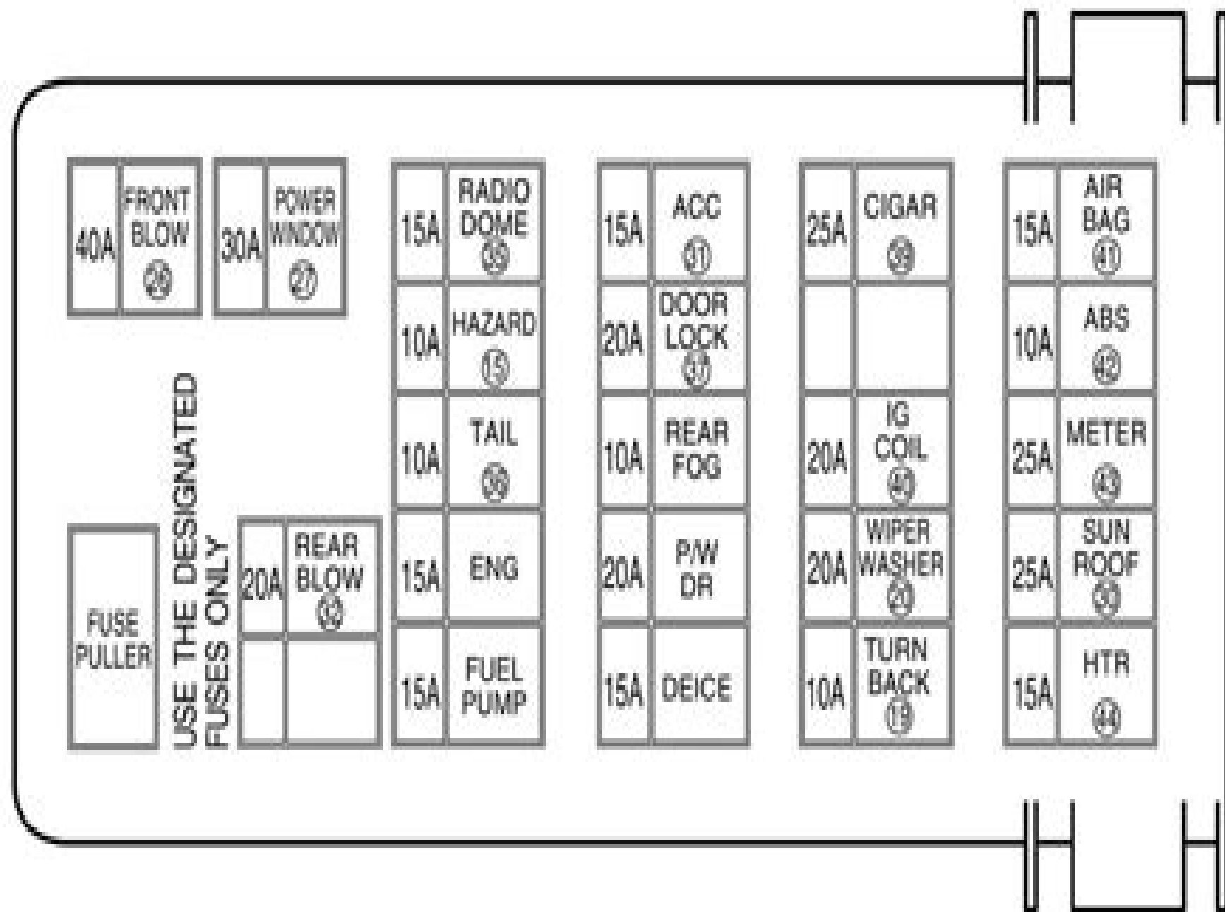
Fig 4. Identifying Passenger Compartment Fuse/Relay Box Components
