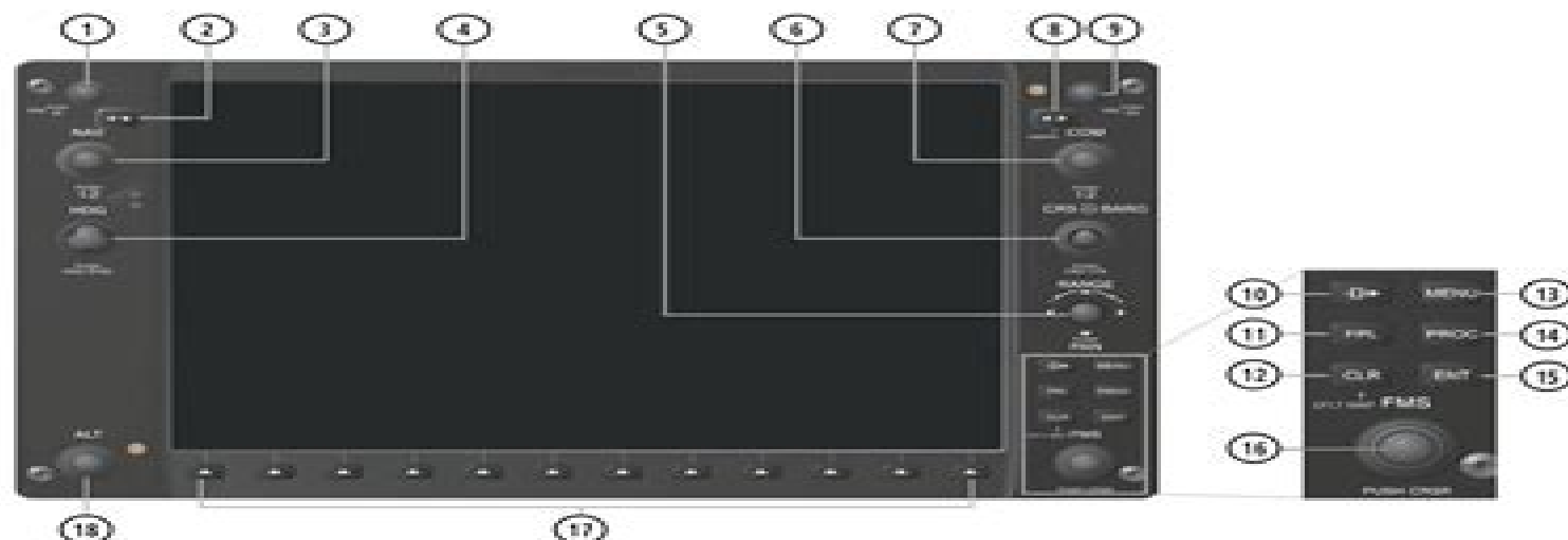
Figure 1-2 PFD/MFD Controls
