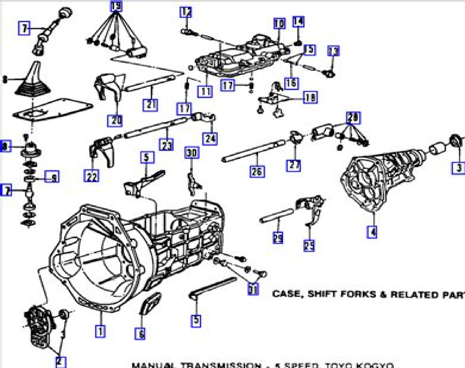
MANUAL TRANSMISSION - 5 SPEED, TOYO KOGYO
