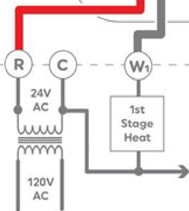
Furnace Connections
