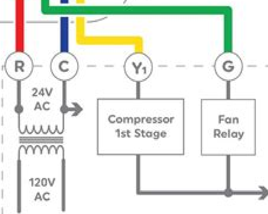
Air Conditioner Connections
