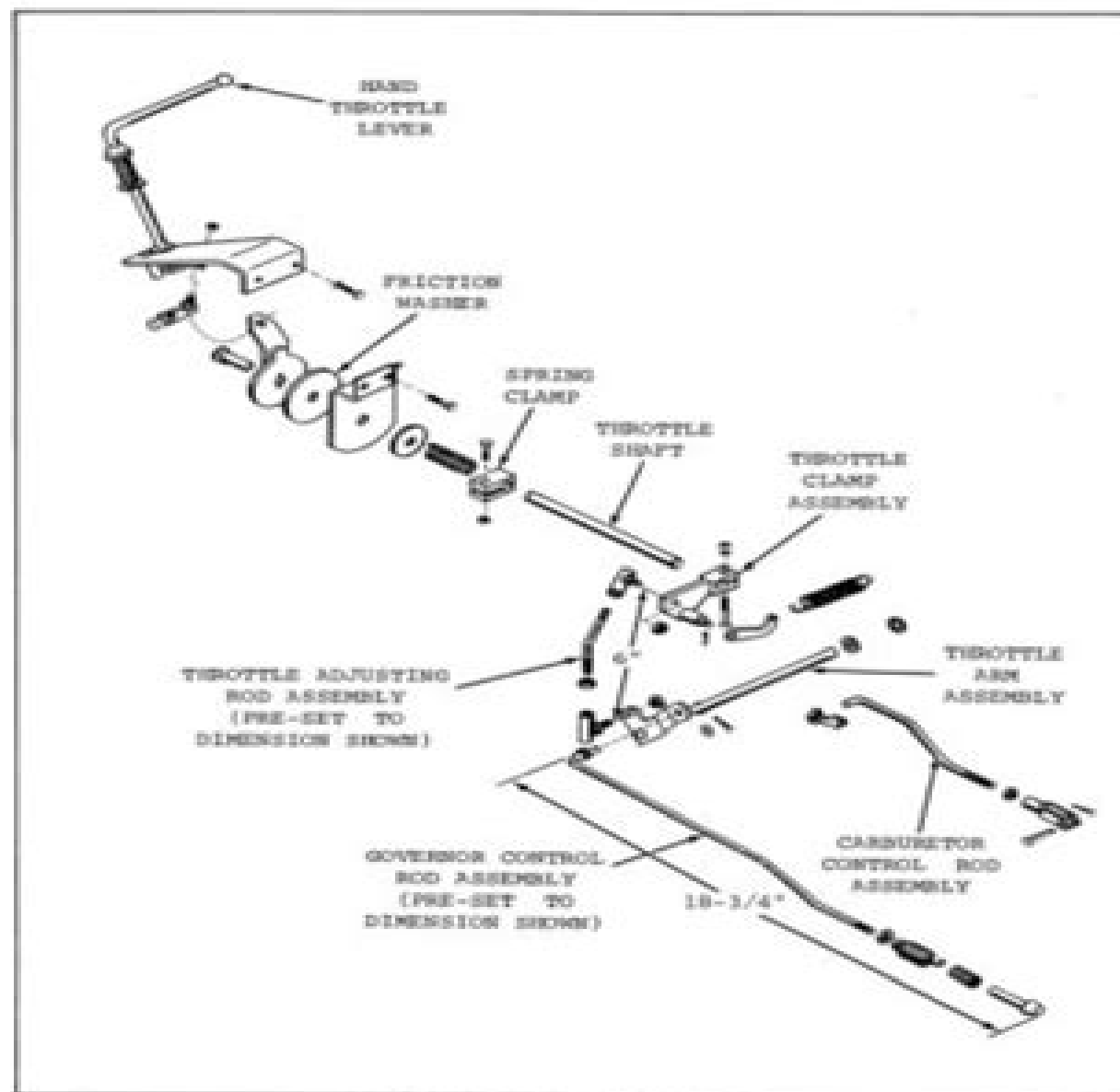
Fig. 2 — Parts Back View of MF 125 Gas Tractor Throttle Linkage
