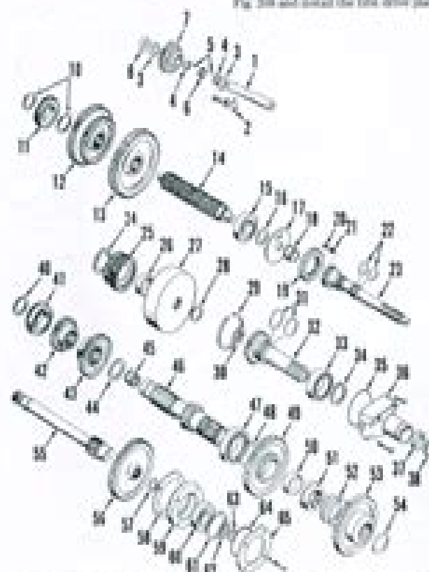
Fig. 205—Exploded view of input shaft, gear and related components used in Multi-Range transmission
