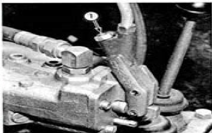
Fig. 17 - Adjustable Detent Mechanism 1. Detent Adjustment Tool
