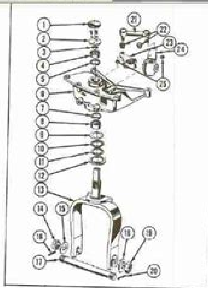
Fig. 8 - Single Front Wheel Axle Nomenclature
