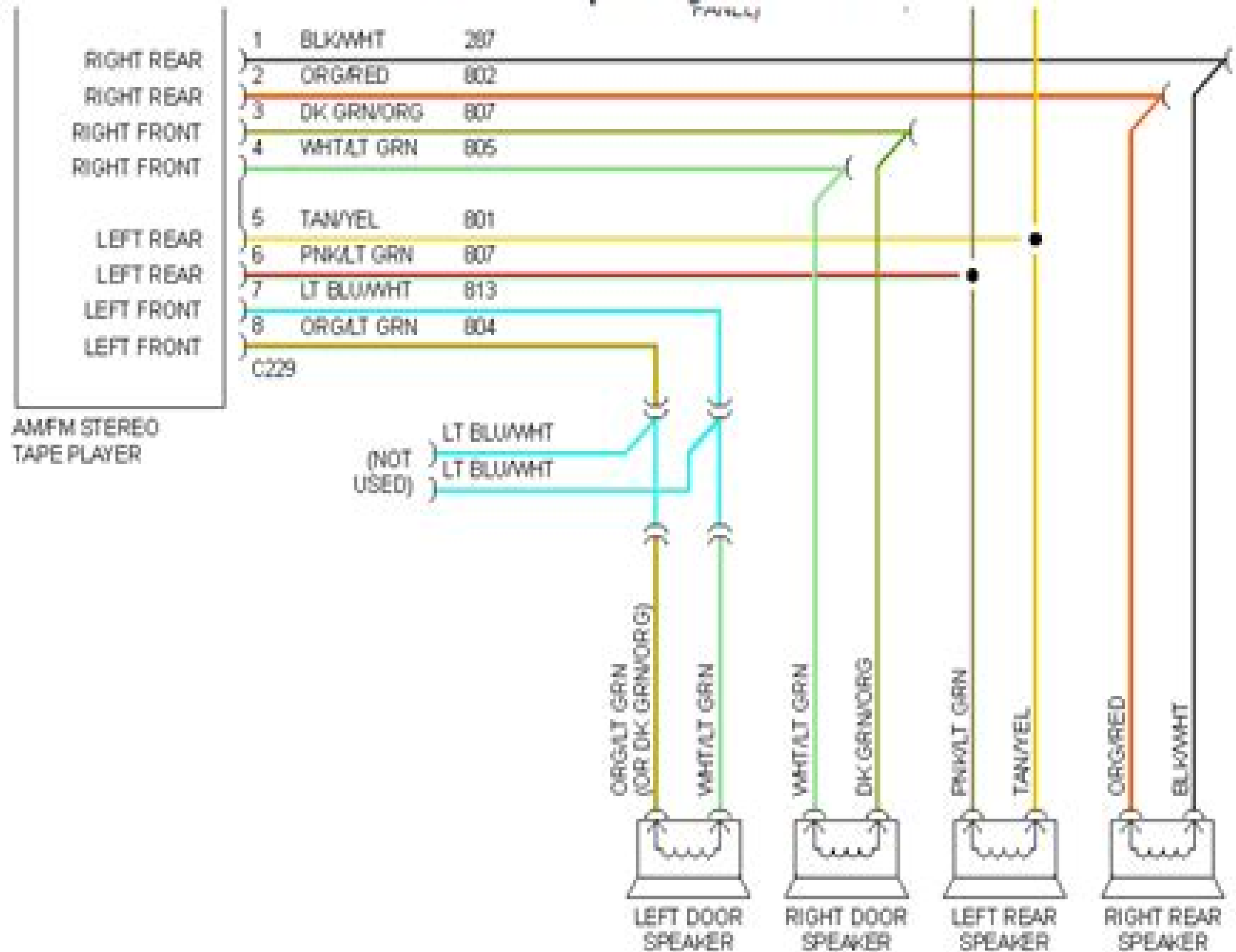
1993 Ford Explorer - Fig. 17: Radio Circuits
