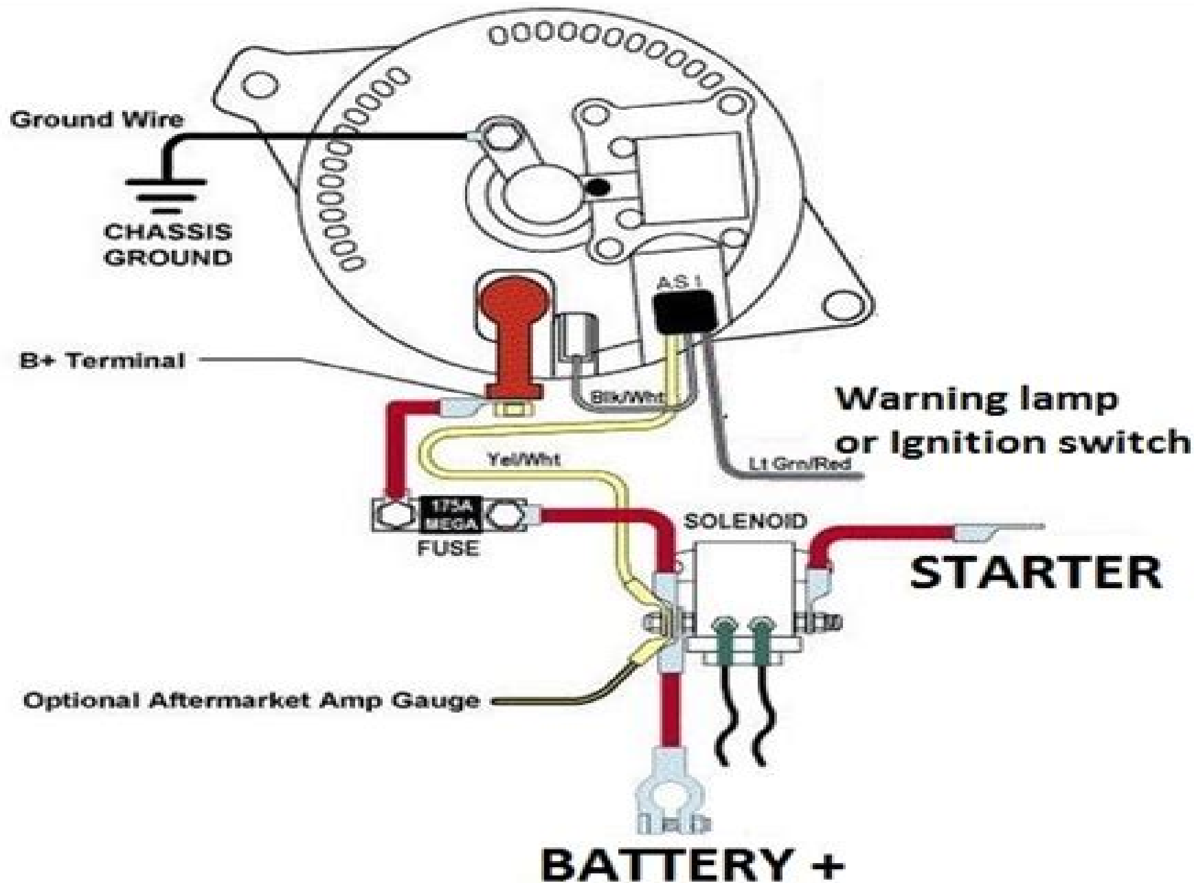
Alternator installation for Mustang 1965
