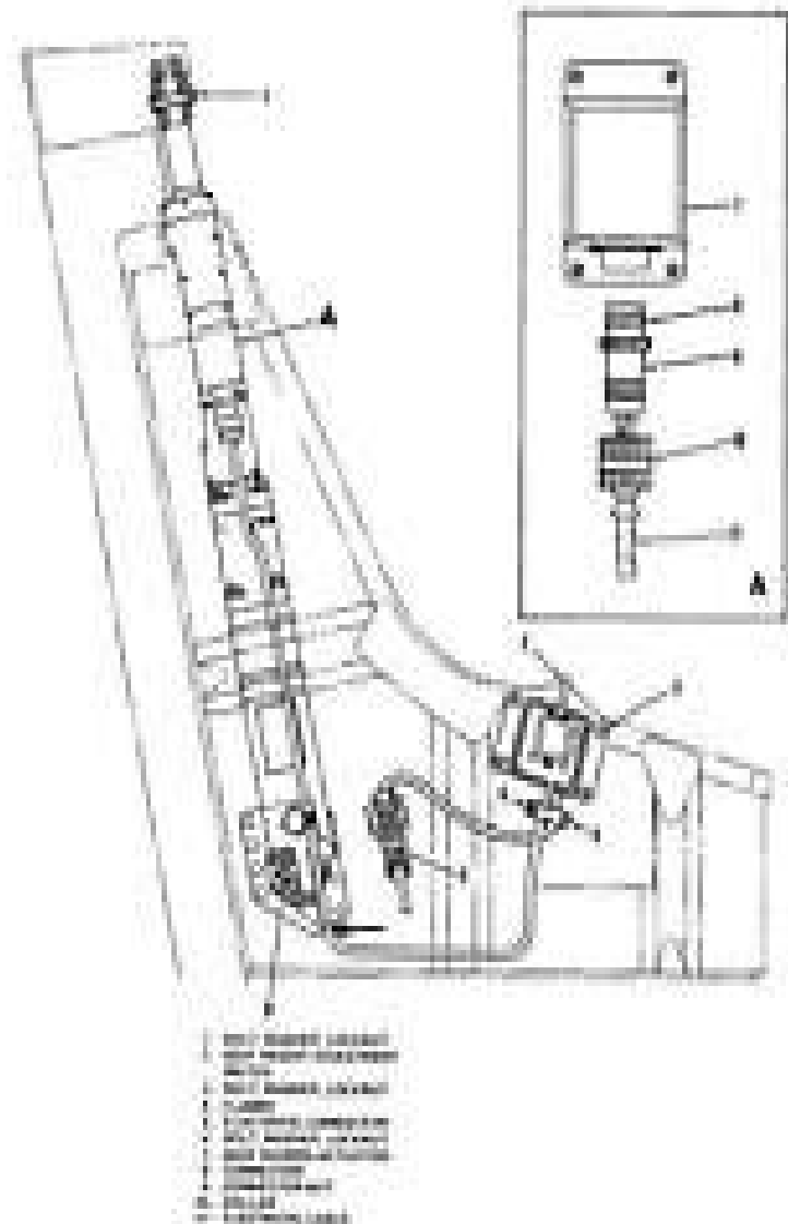
Figure 4-4. Fuel system part identification
