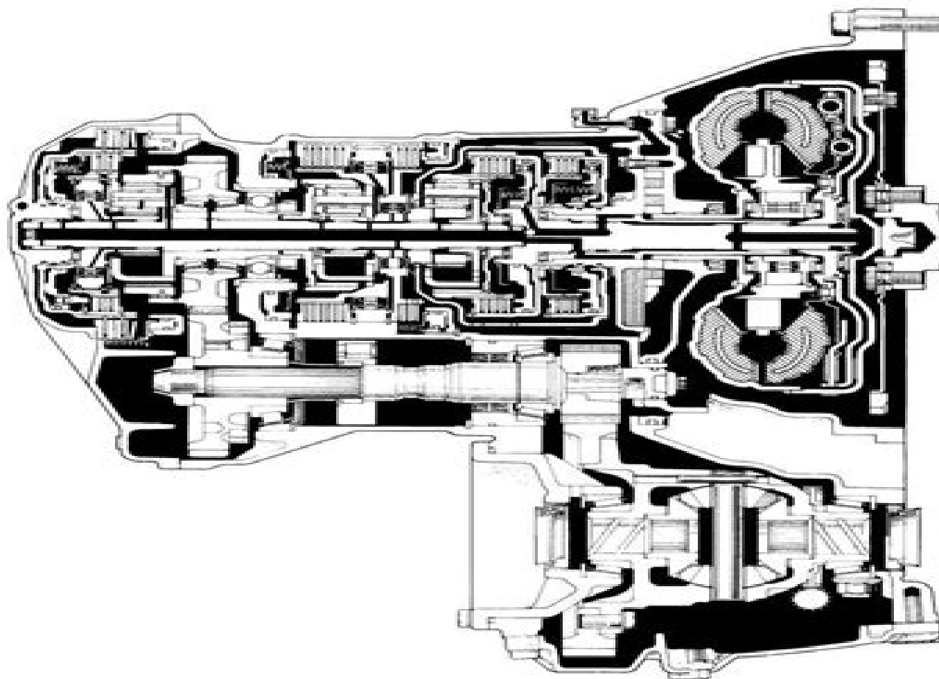
Sectional View
