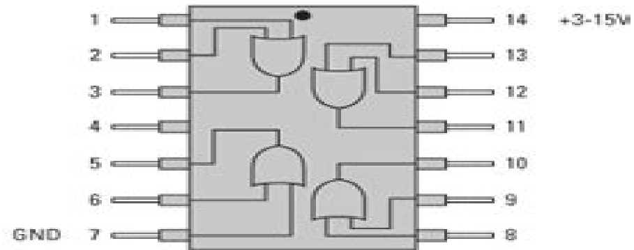
4071 Quad OR
