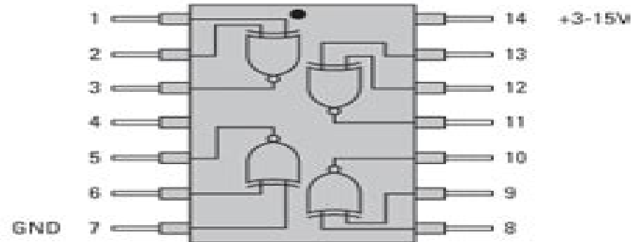
4077 Quad XNOR
