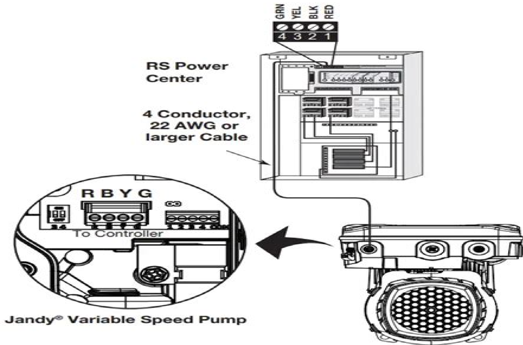
Figure 14. Low Voltage Wiring for Jandy Variable Speed Pump
