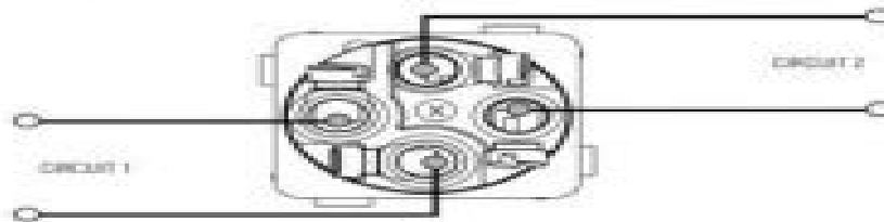
Changeover Switch Mechanism, 10A, 250V a.c.
