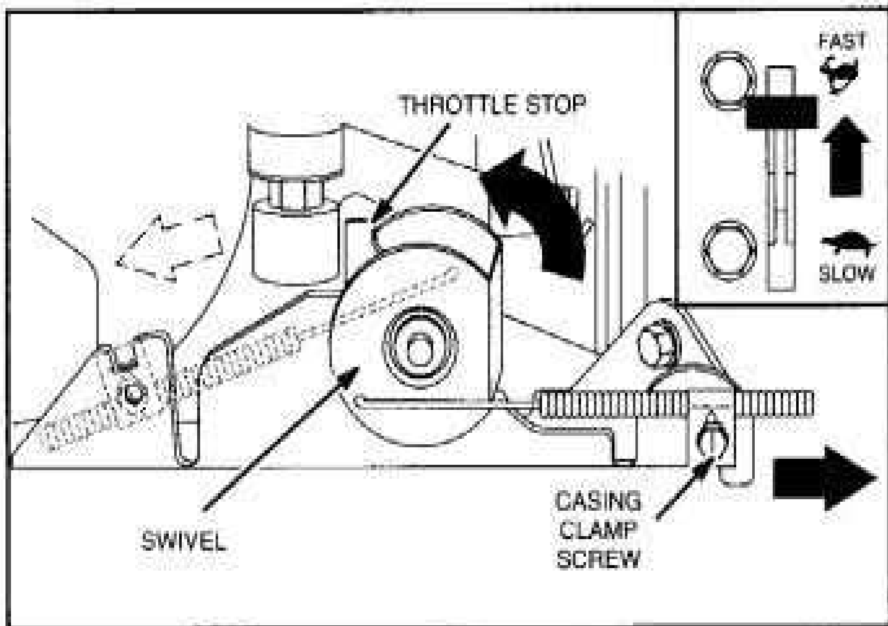
Fig. 4 – Control Wire Adjustment
