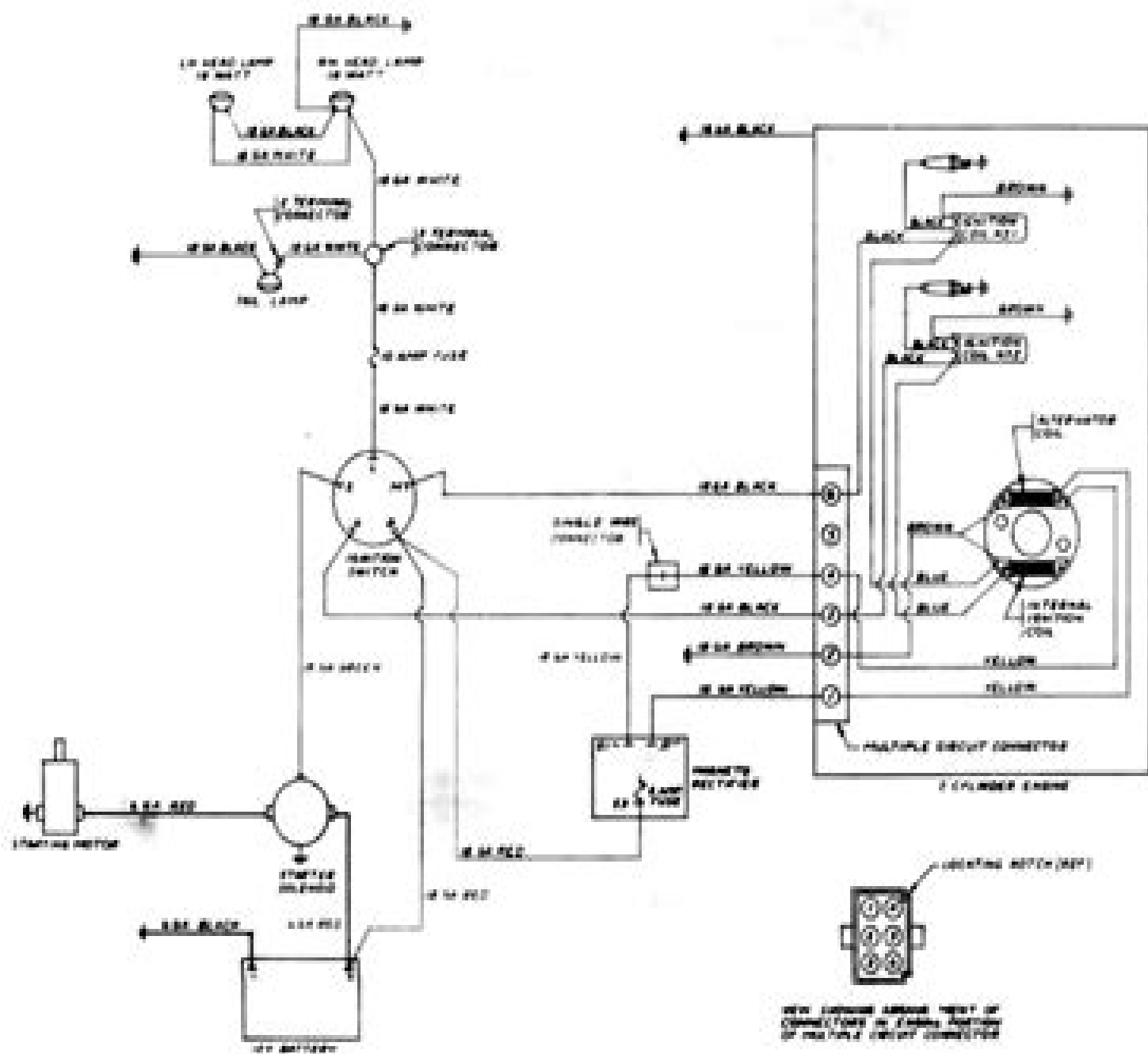
Fig. 28 - Schematic - Electric Start Wiring - Model 500 SST
