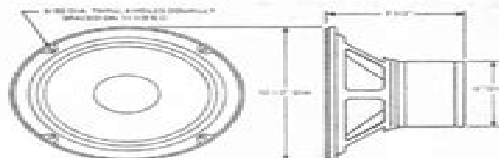
Figure 1 Dimensions
