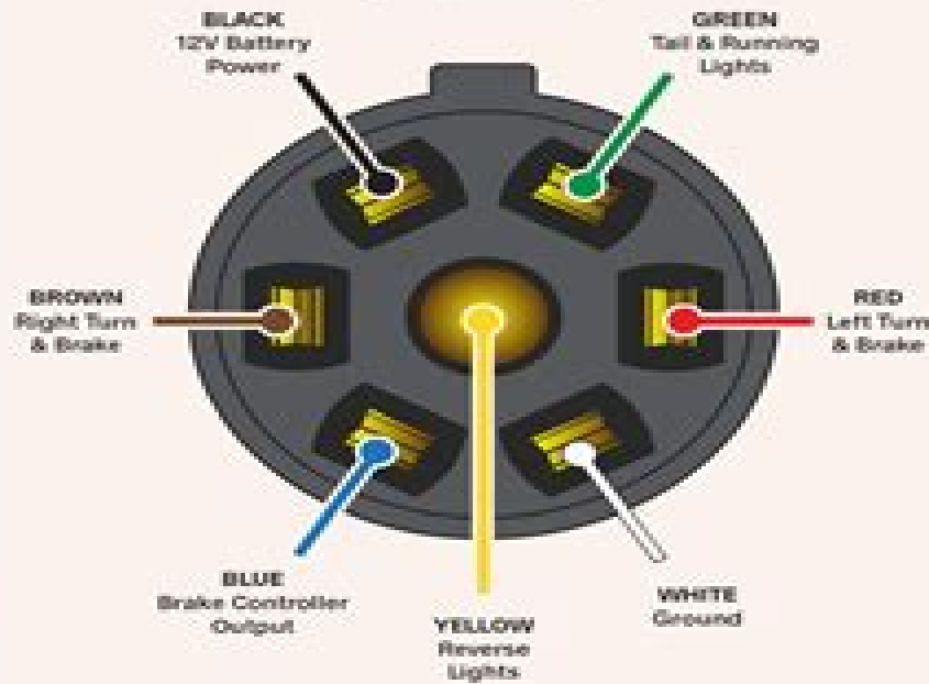
Plug Side
