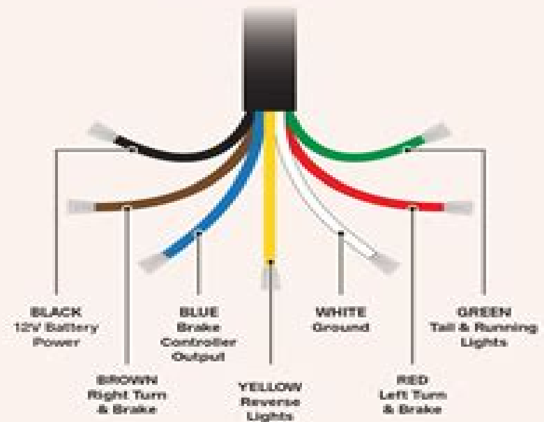
Wiring Side
