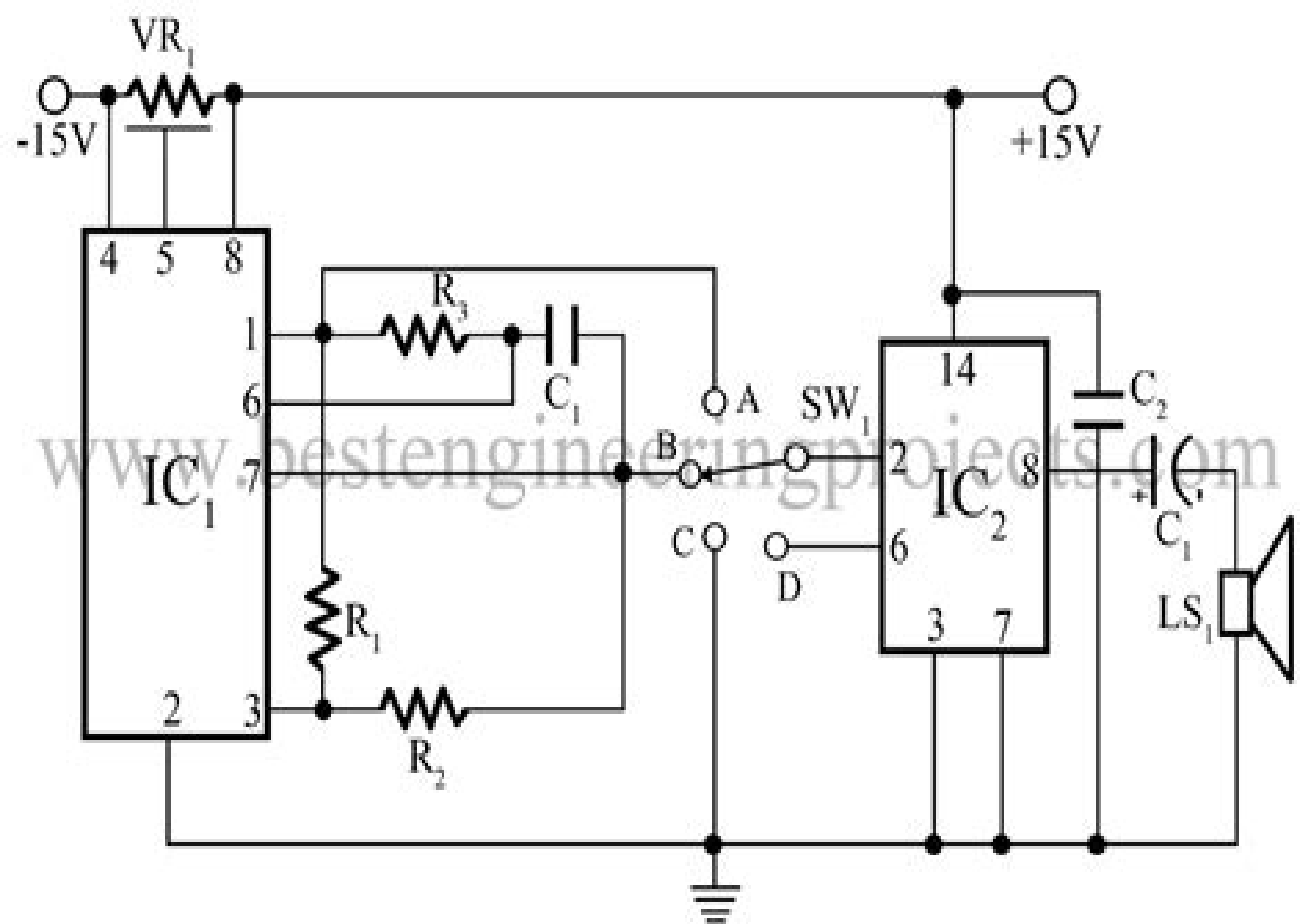
Figure 1: Circuit Diagram of Electronic Siren Circuit
