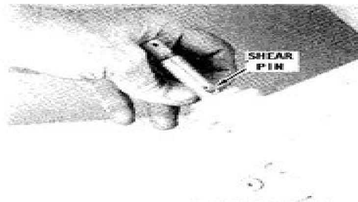
Shear-pin installed behind the propeller instead of in front of the propeller.
