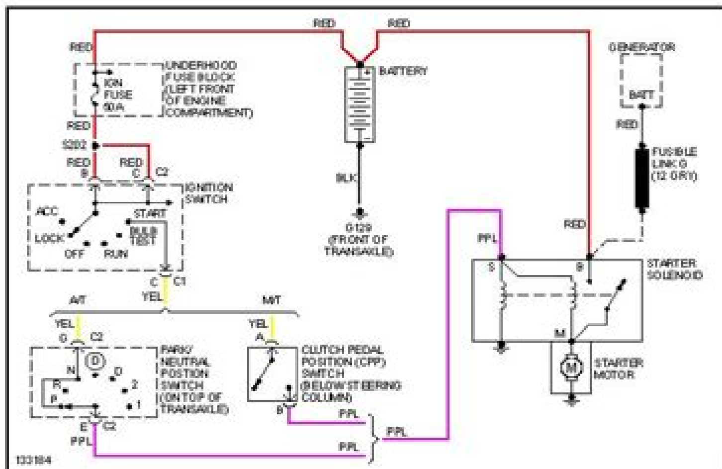
2000 Chevrolet Cavalier-Fig. 5: Starting System Wiring Diagram (Cavalier & Sunfire)
