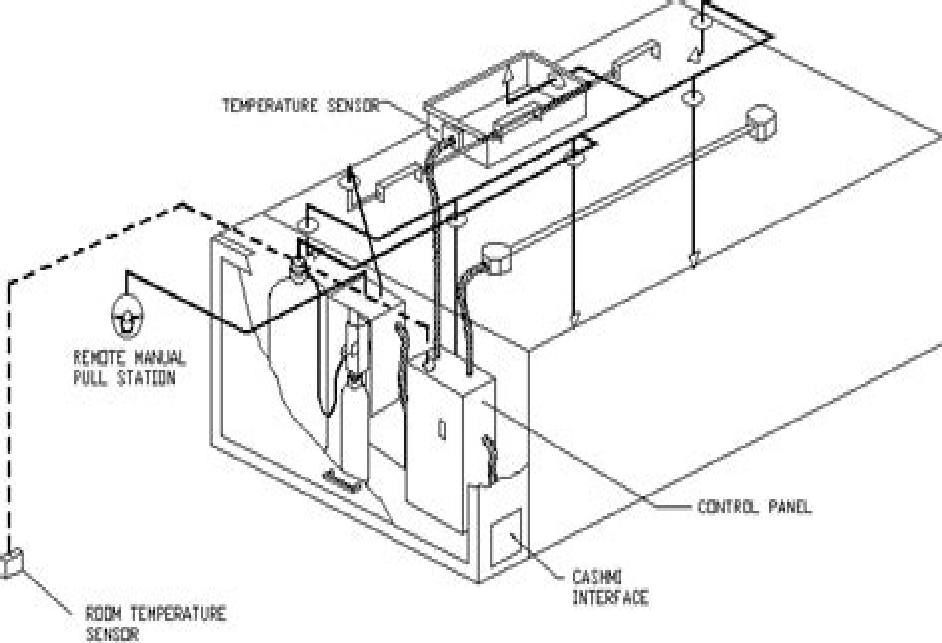
TYPICAL CONTROL CENTER INSTALLATION
