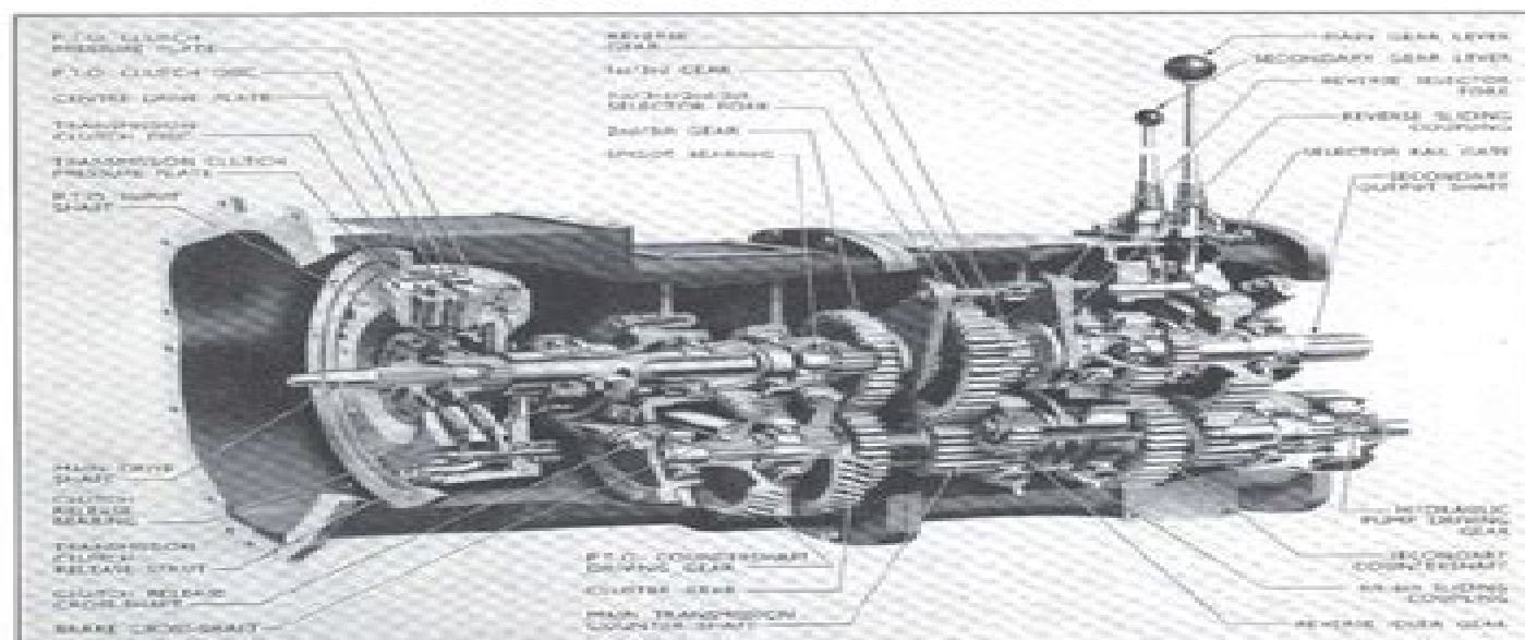
Fig. 1 Sectioned Gearbox
