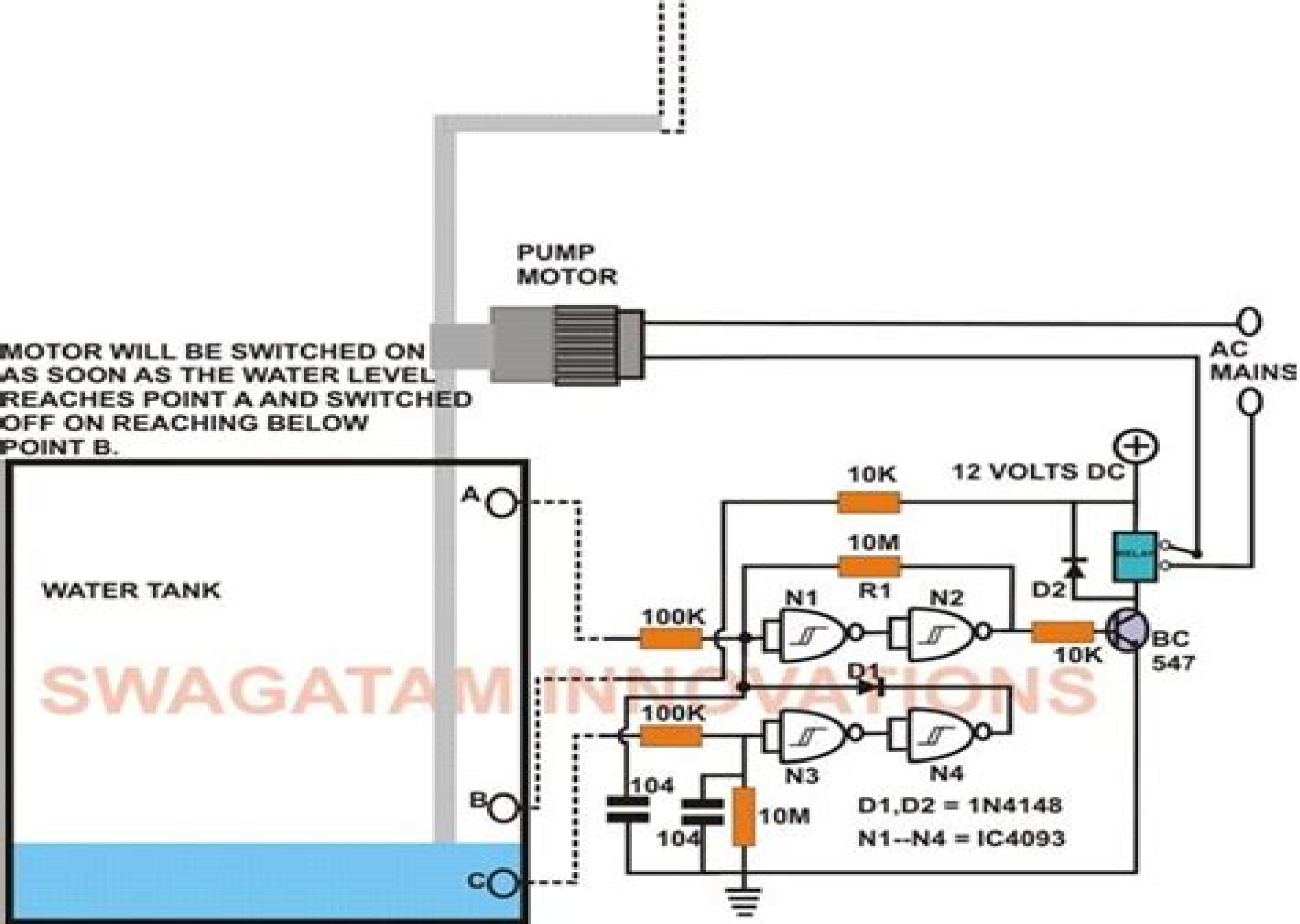
AUTOMATIC WATER LEVEL CONTROLLER CIRCUIT SCHEMATIC
