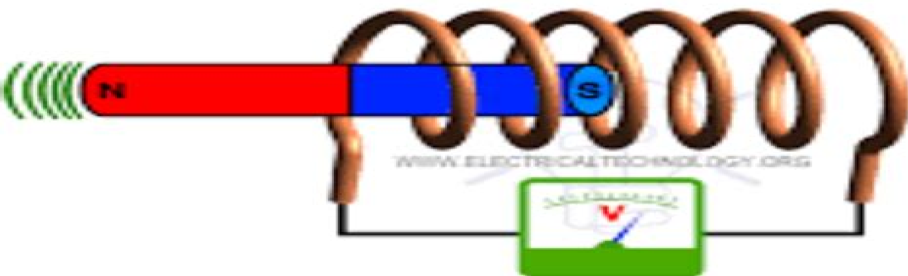
Fig 1.B: As magnet moves more rapidly to the right, magnetic field is changing more rapidly with respect to the coil and a greater EMF is induced.
