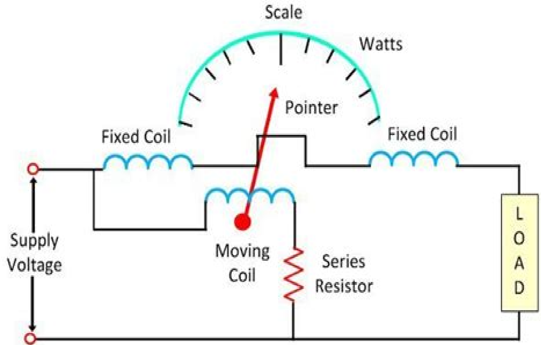
Electrodynamometer Wattmeter
