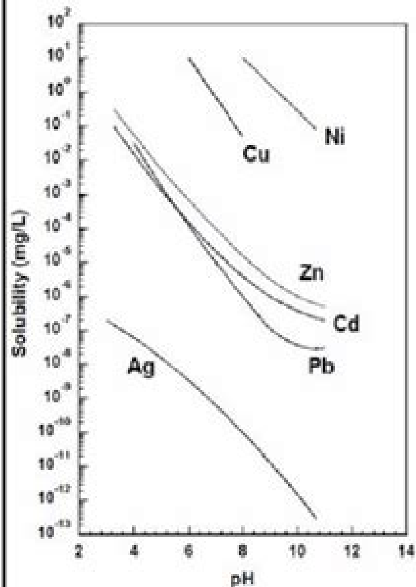
Metal sulphide
