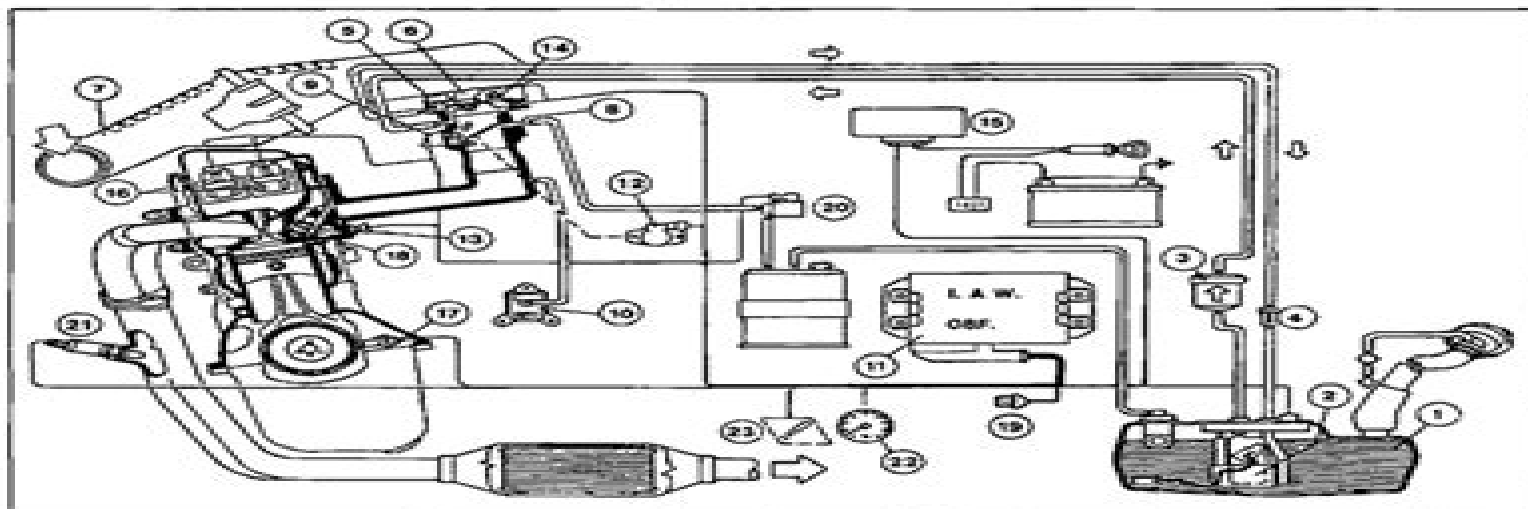
1.1 IAW Weber-Marelli single point injection (SPI) system
