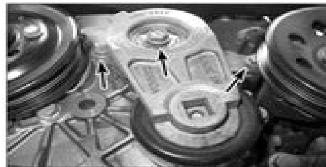
24.25 Typical V8 tensioner mounting fastener locations
