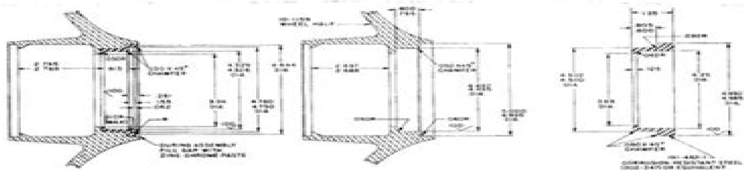
Figure 6. Repair of Outer Wheel Half Bearing Bore and Lock Ring Groove
