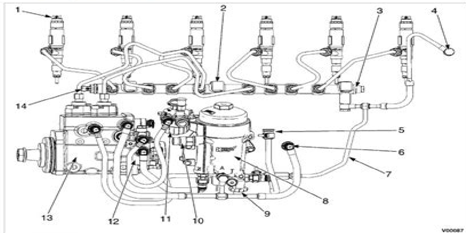
Figure 16 Fuel system
