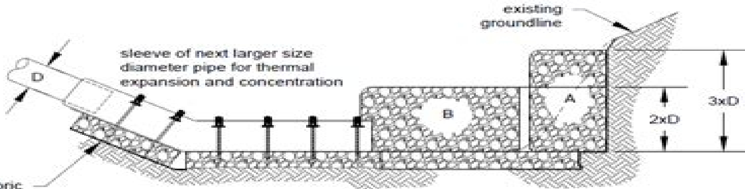
Section C-C
