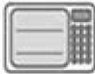
MICROWAVES
