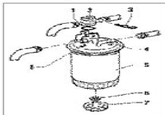
23.3 Fuel filter details
