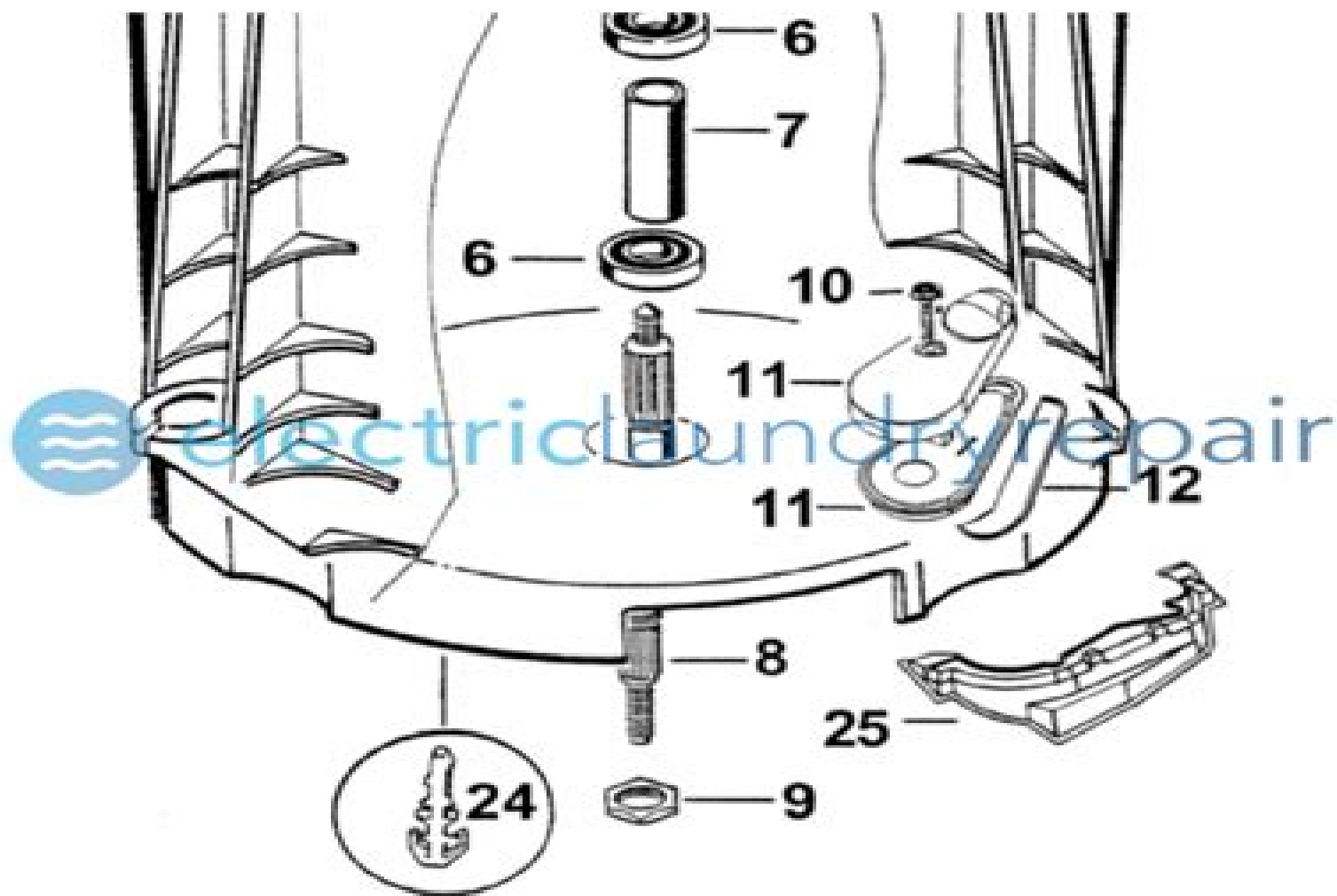
Item #8 - Shaft, Drive
