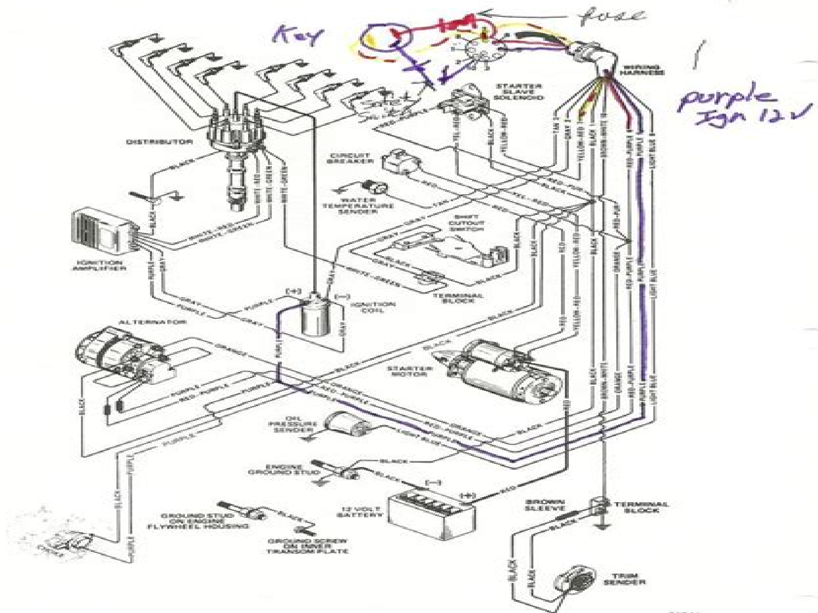
MCM 200 5.0 Litre Engine (Battery Meter Circuit)
