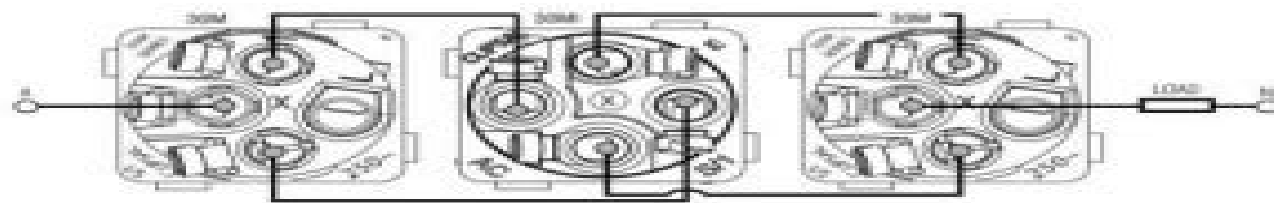
Intermediate Switch Mechanism, 10A, 250V a.c.
