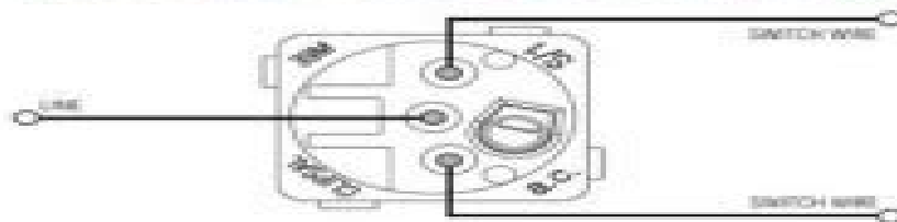
Three Position Switch Mechanism, Marked HI-OFF-LO
