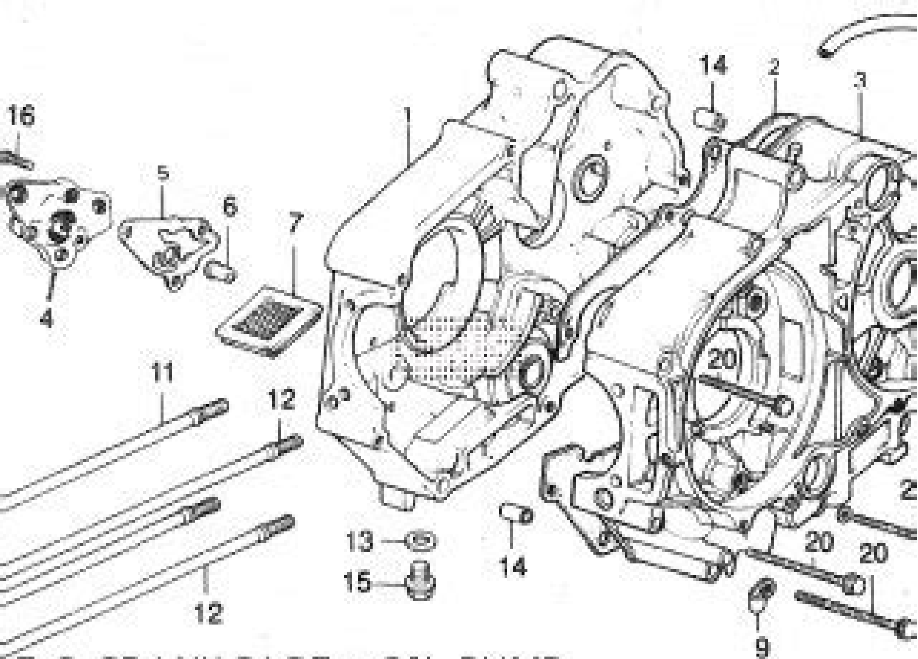
E-8 CRANK CASE - OIL PUMP
